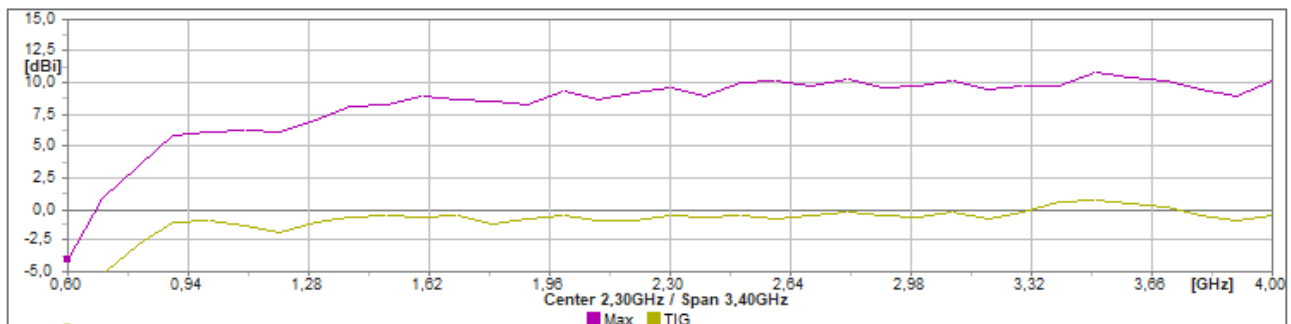
3D Gain
